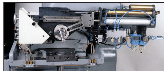
Pneumatic Infeed Attachment
